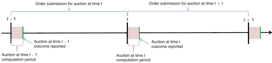
FIGURE 1. PROCESS FLOW FOR FREQUENT BATCH AUCTIONS
