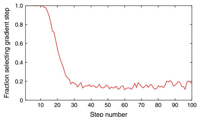
Figure 6. (Color online) The average fraction of search steps that selected a gradient neighbor (i.e., \bar{p} is of the gradient neighbor type in line 20 of Algorithm 1) at a given number of steps in the spring 2014 Course Match production run
